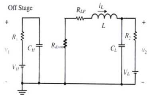
Figure 9. Snubber circuit.
