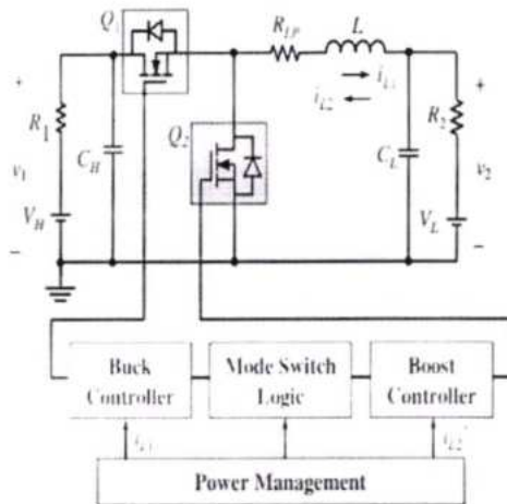
Figure 11. Individual controllers.
