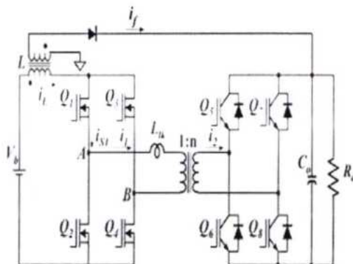
Figure 3. Isolated converter.
