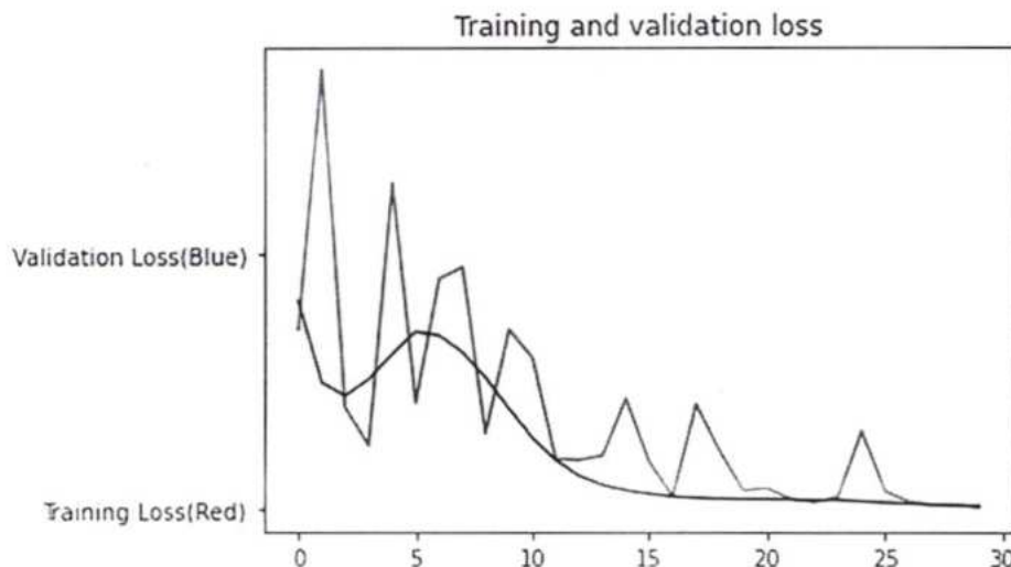
Fig. 17. Training loss Vs validation loss using EfficientNet model.
